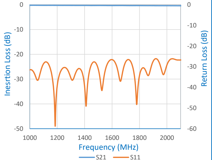
FREQUENCY VS INSERTION LOSS
