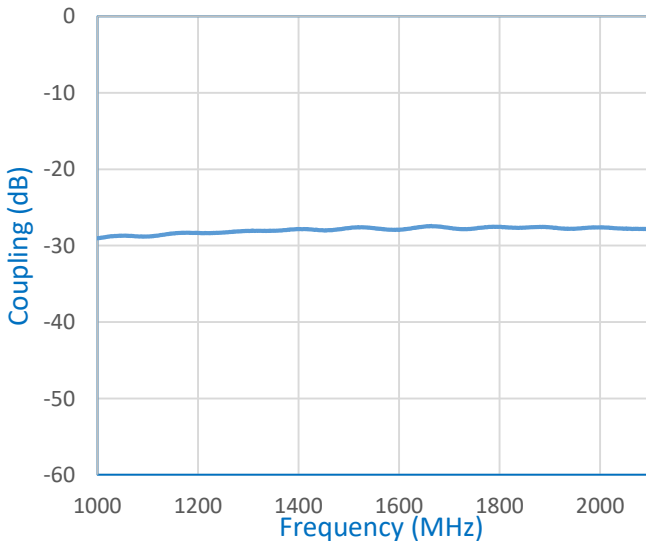
FREQUENCY VS COUPLING
